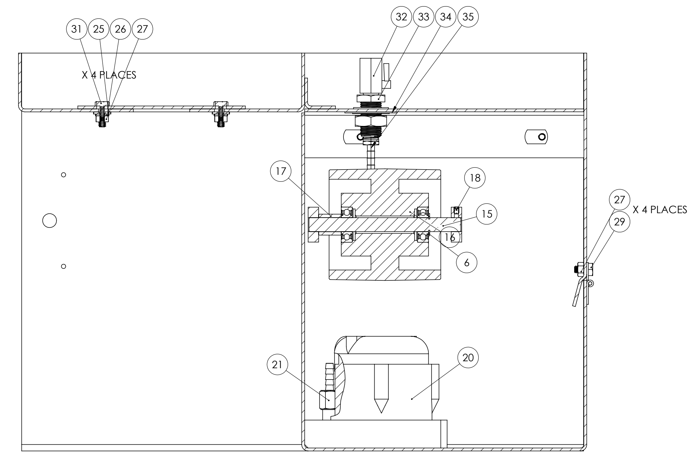
SECTION B-B SCALE 1:2 IDLER PULLEY INTERNAL VIEW
