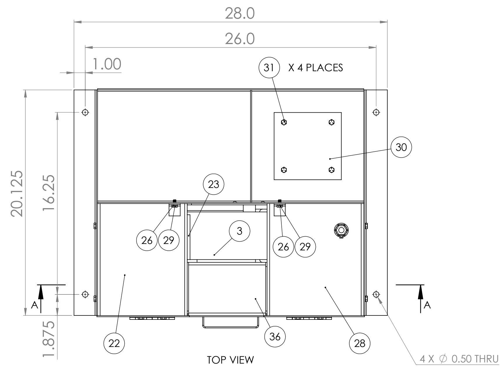
TOP VIEW
