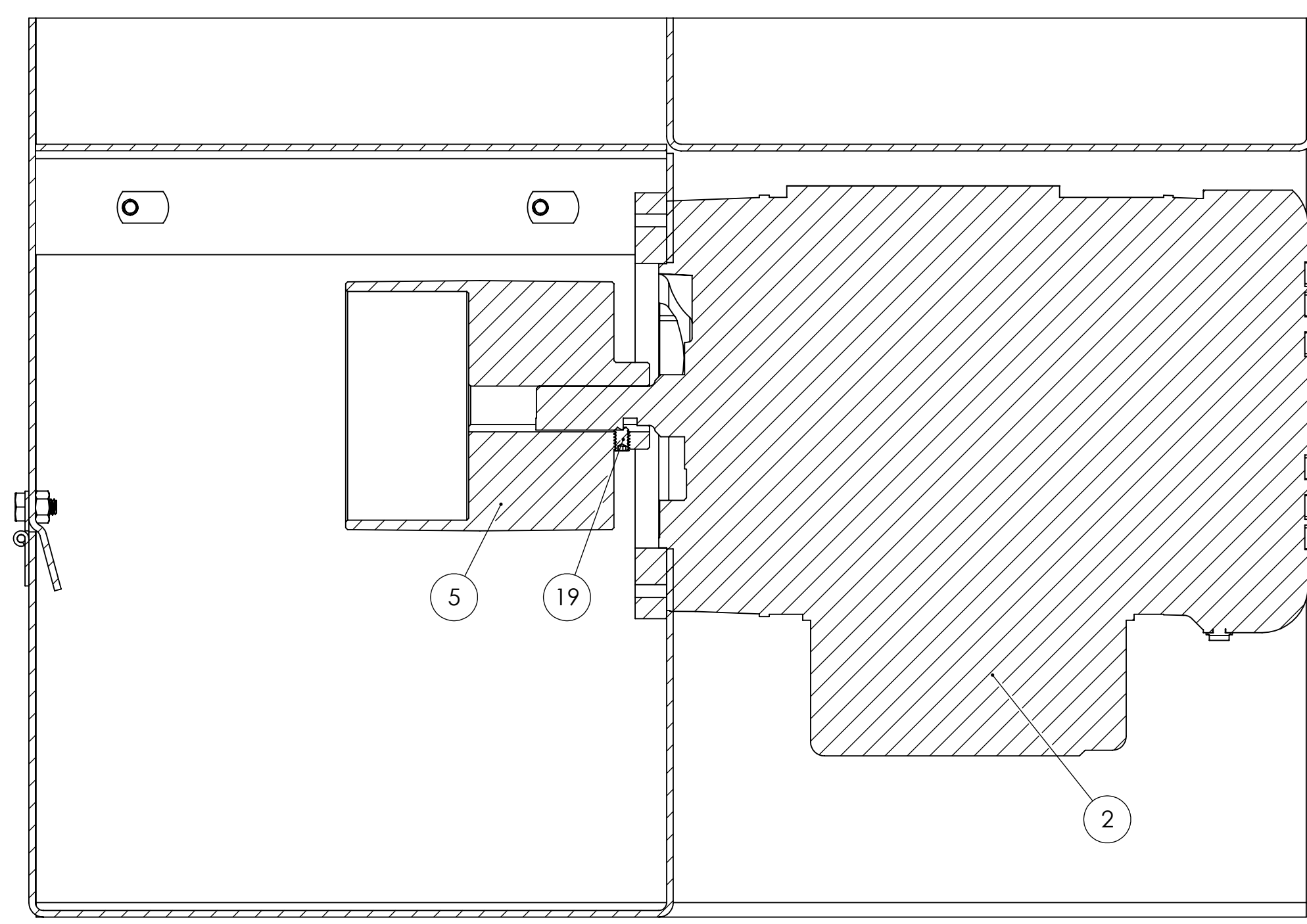
SECTION C-C SCALE 1:2 DRIVE PULLEY INTERNAL VIEW
