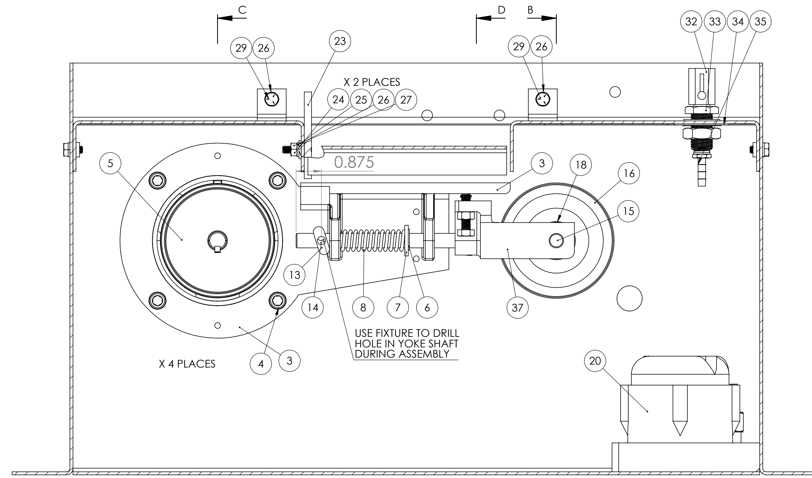
SECTION A-A SCALE 1:2 MAIN INTERNAL VIEW
