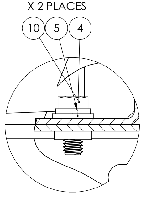
DETAIL B SCALE 1 : 1 DISC GUARD FASTENER DETAILS
