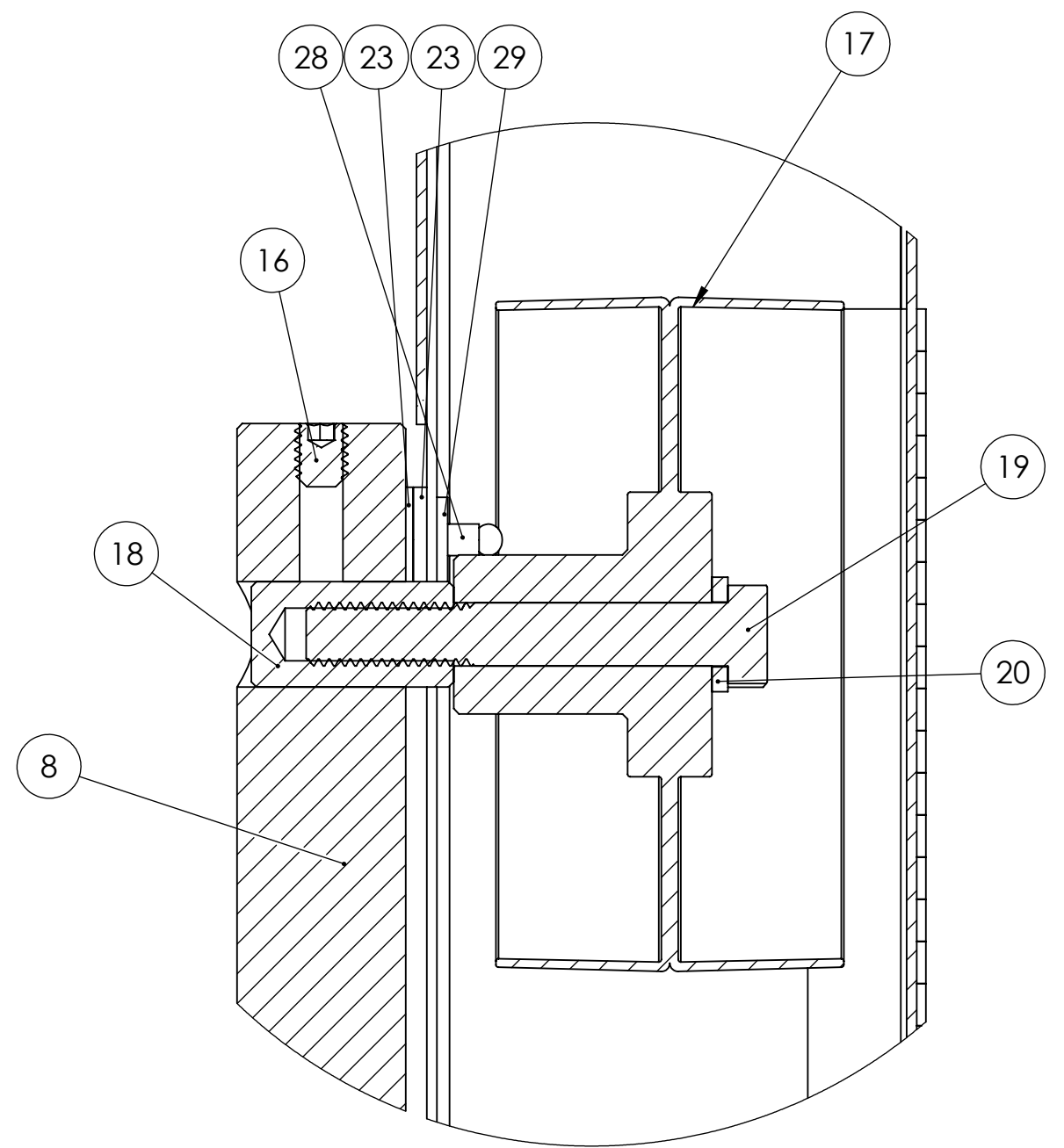
DETAIL B SCALE 1 : 1 IDLER PULLEY DETAIL
