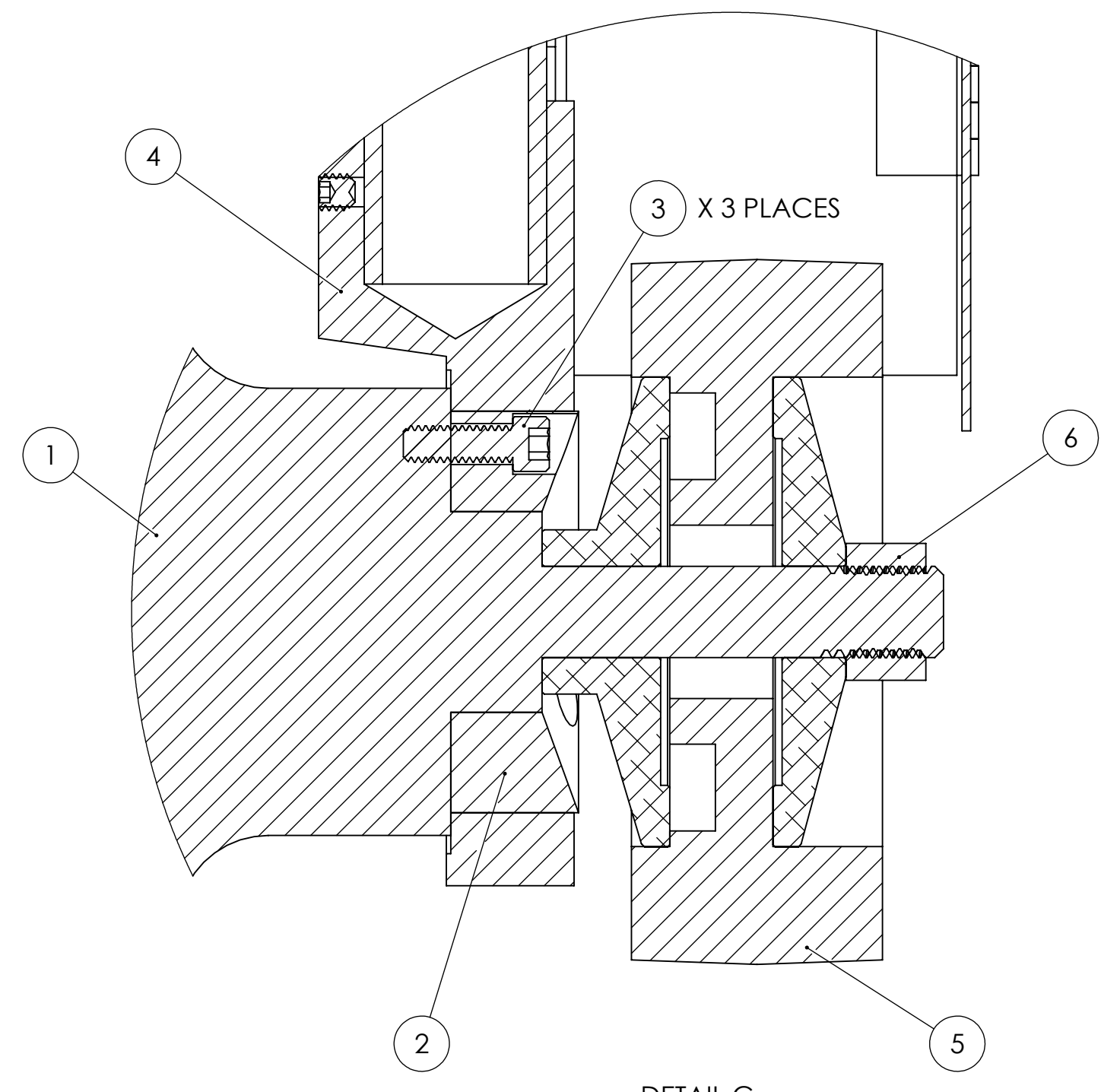
DETAIL C SCALE 1 : 1 DRIVE PULLEY DETAIL
