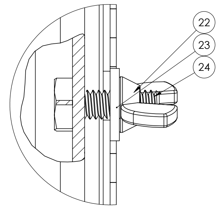
DETAIL D SCALE 2 : 1 BELT GUARD LATCH DETAILS
